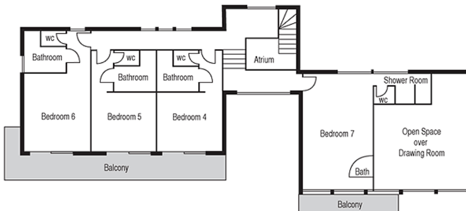
First Floor
